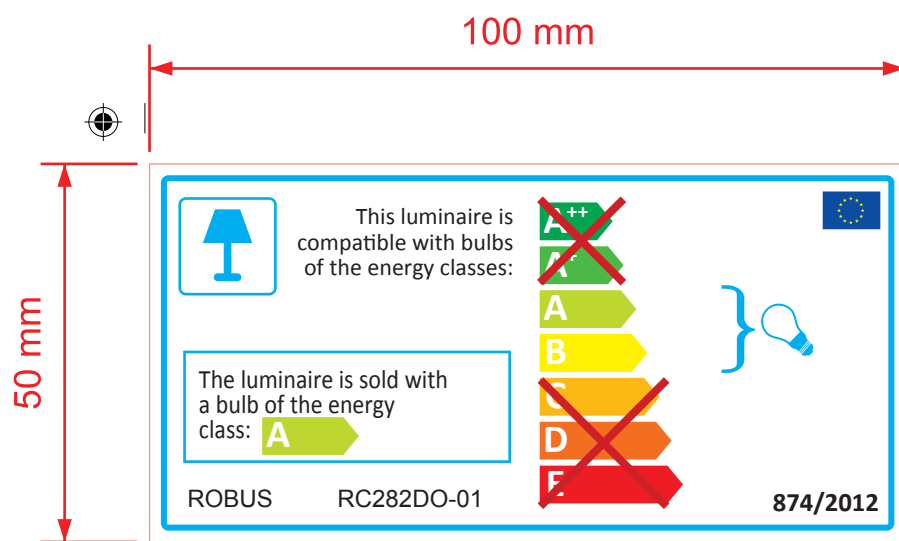
LEL-08 (Mono-L) - UK 50mm x 100mm
