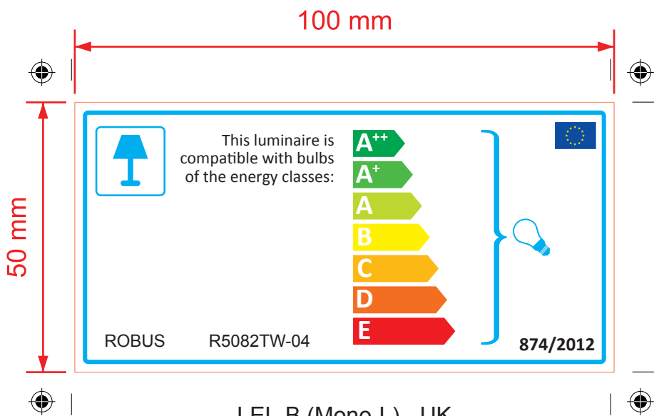
LEL-B (Mono-L) - UK 50mm x 100mm
